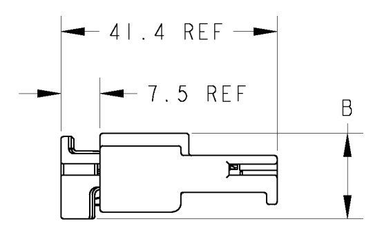
ENGAGEMENT VIEW 嵌合状態 SCALE 1:1
